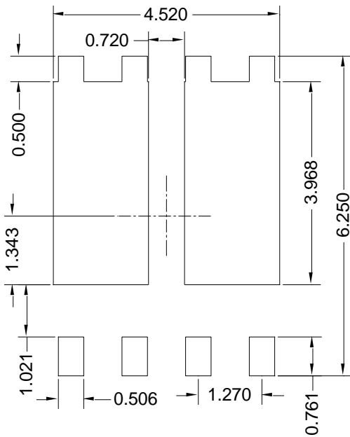
Suggested Solder Pad Layout Top View
