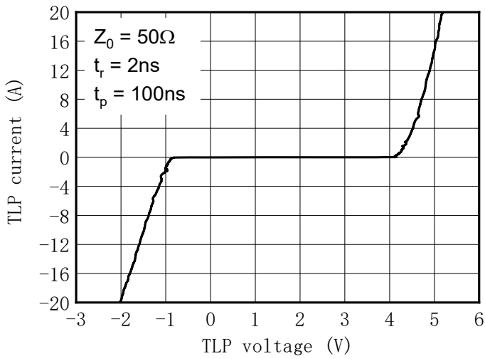
Fig.9 TLP Measurement
